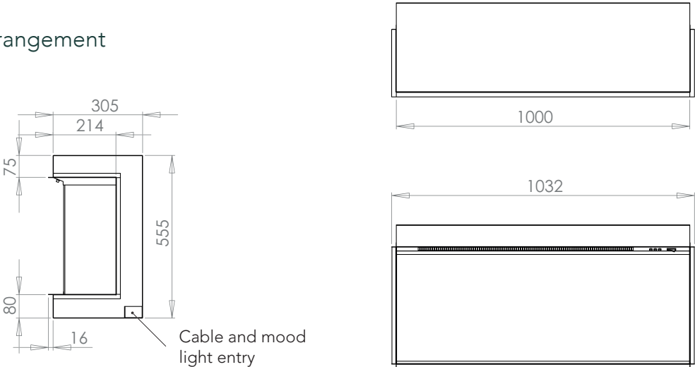
i1250e Deep Three-sided arrangement
